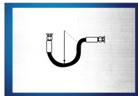
Illustrations 3: The bend radius can not be less than the minimum bend radius
